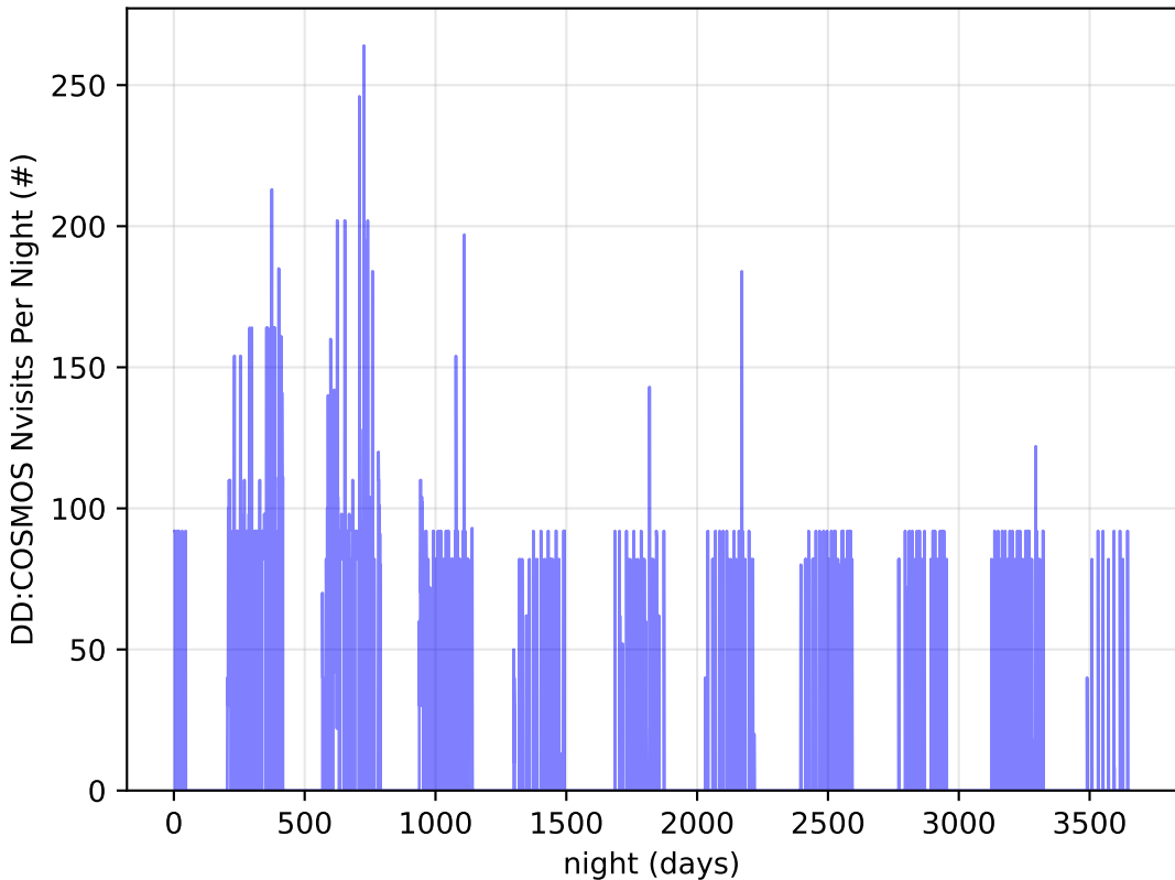
noroll_mjdp0_v3.4_10yrs all bands: DD:COSMOS Nvisits Per Night
