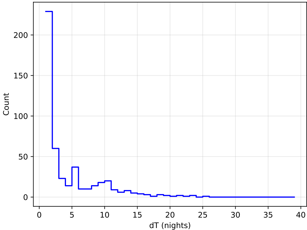
noroll_mjdp0_v3.4_10yrs all bands: DD:COSMOS Delta Nights Histogram
