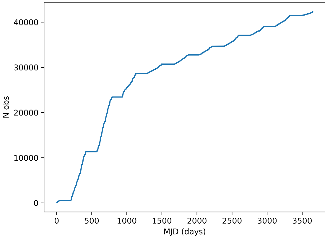
noroll_mjdp0_v3.4_10yrs all bands: DD: COSMOS Cumulative NVisits
