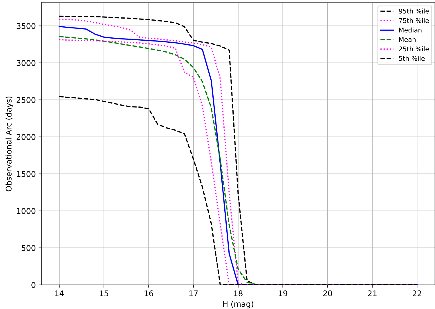
no_magell_roll_v3.4_10yrs: Observational Arc Length Trojan
