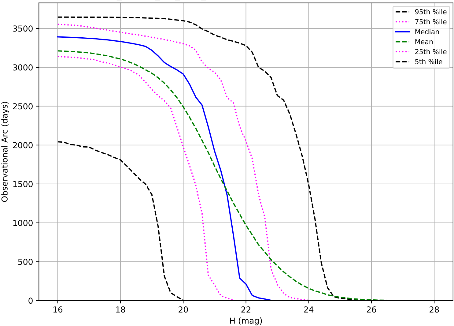
no_magell_roll_v3.4_10yrs: Observational Arc Length PHA
