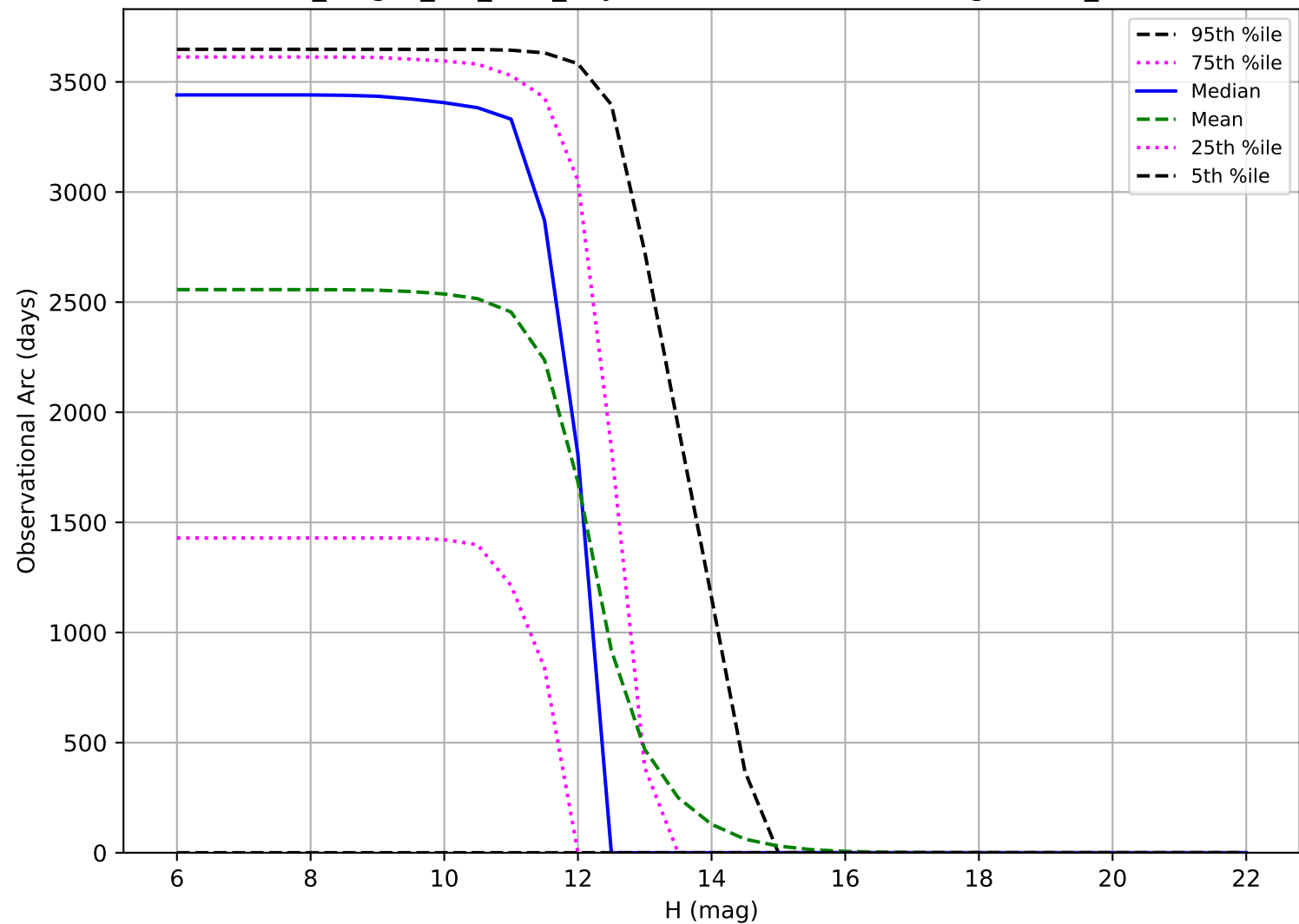
no_magell_roll_v3.4_10yrs: Observational Arc Length OCC_r20
