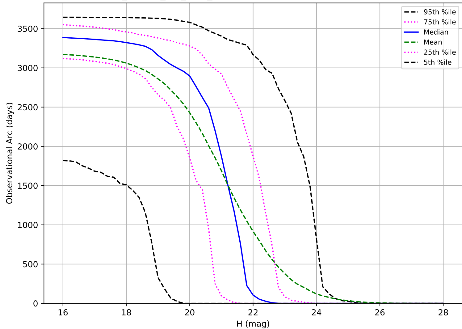
no_magell_roll_v3.4_10yrs: Observational Arc Length NEO
