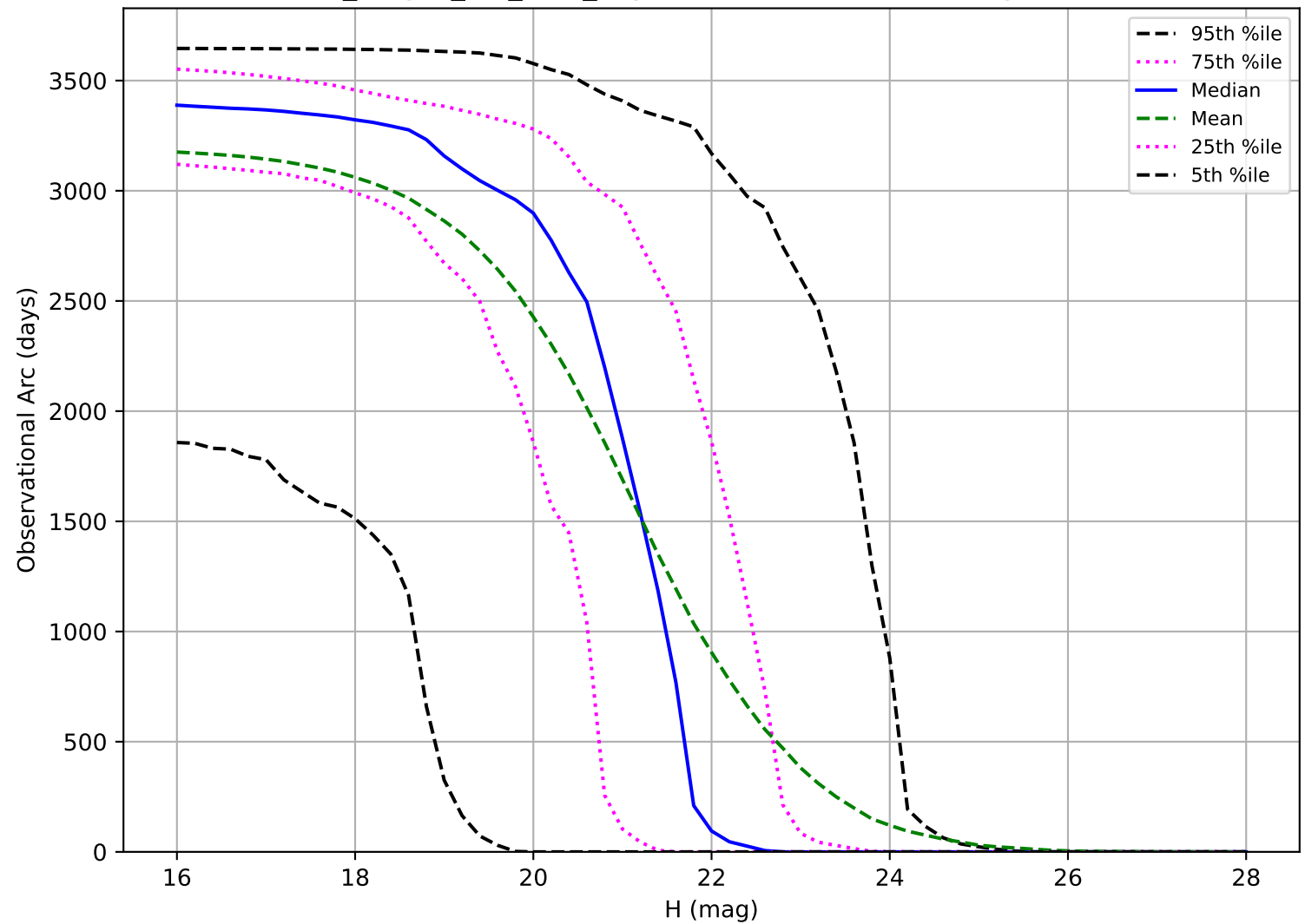
no_magell_roll_v3.4_10yrs: Observational Arc Length NEO
