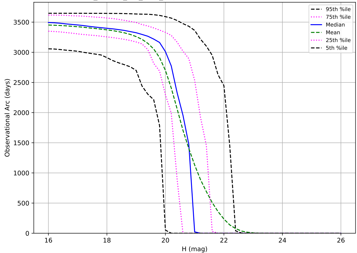
no_magell_roll_v3.4_10yrs: Observational Arc Length MBA
