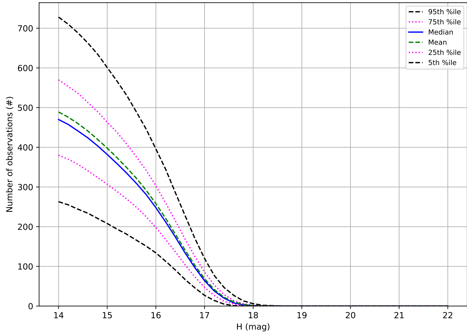
no_magell_roll_v3.4_10yrs: Number of observations Trojan
