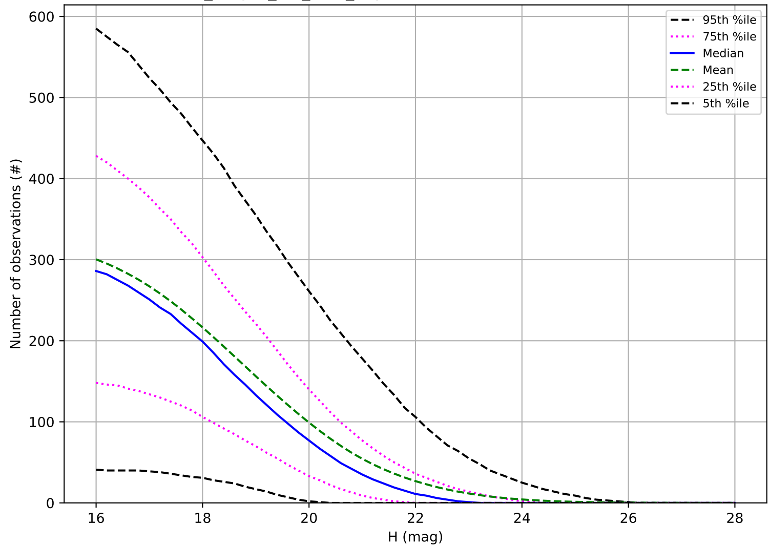
no_magell_roll_v3.4_10yrs: Number of observations PHA
