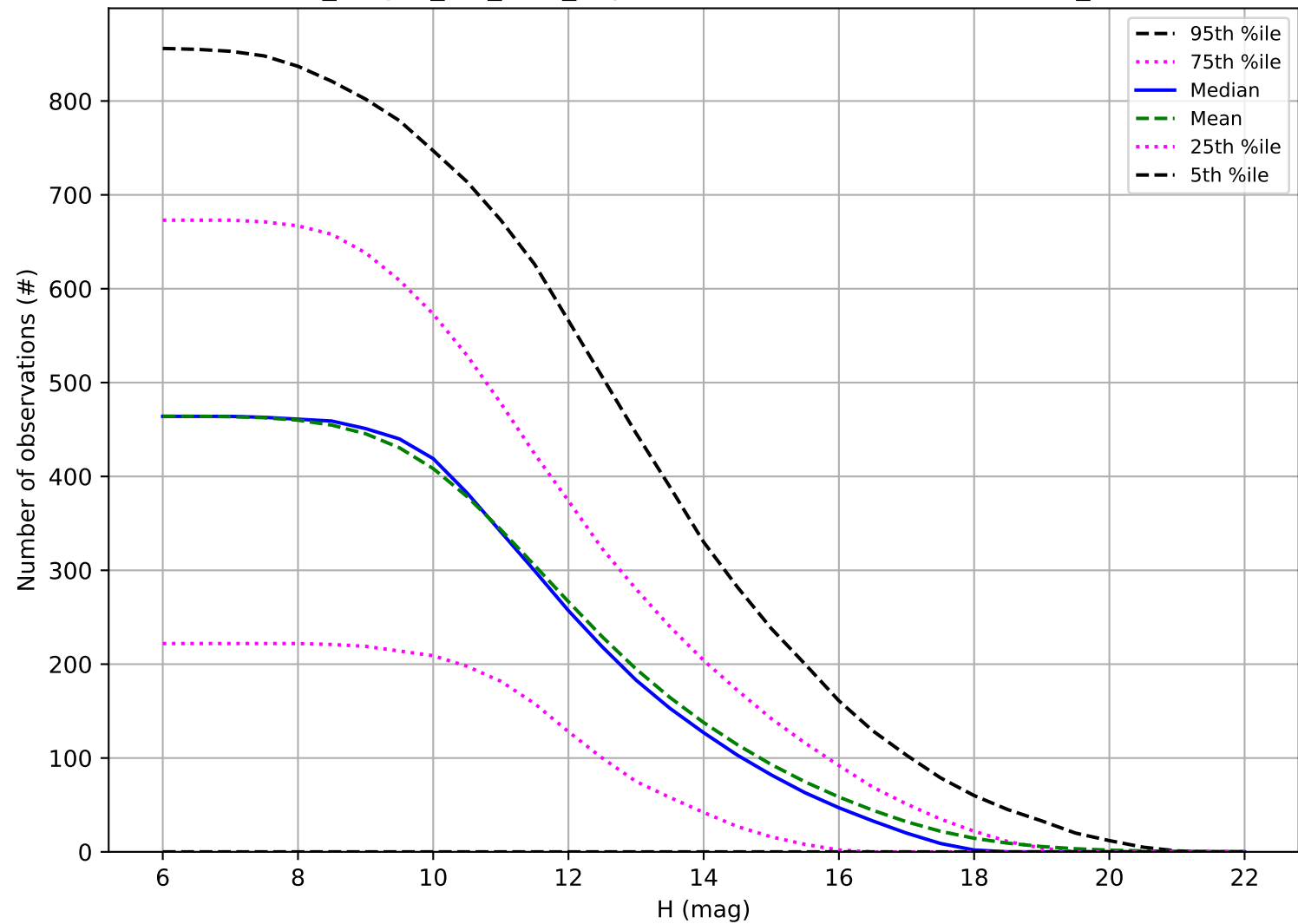
no_magell_roll_v3.4_10yrs: Number of observations OCC_r5
