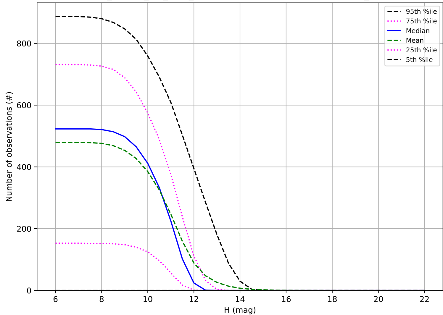
no_magell_roll_v3.4_10yrs: Number of observations OCC_r20
