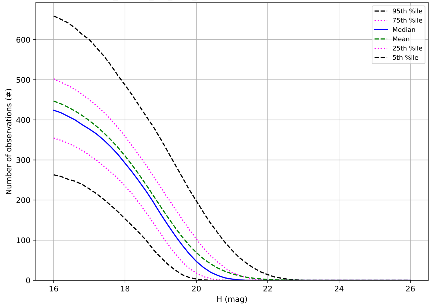
no_magell_roll_v3.4_10yrs: Number of observations MBA
