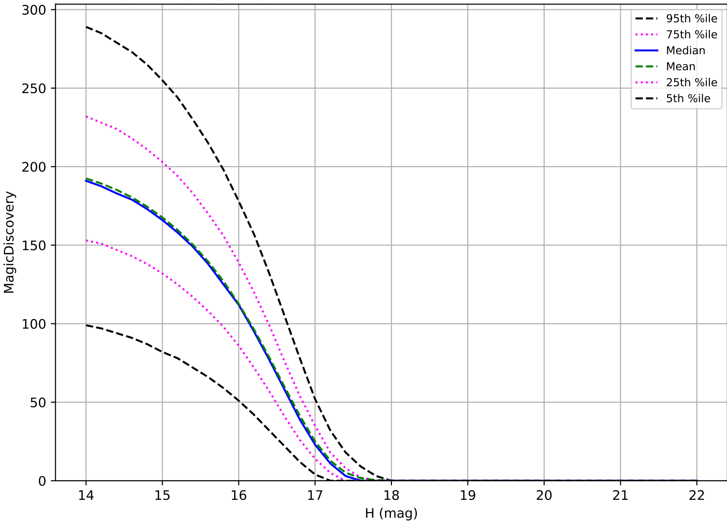
no_magell_roll_v3.4_10yrs: Trojan 6 detections in 60 nights detection loss
