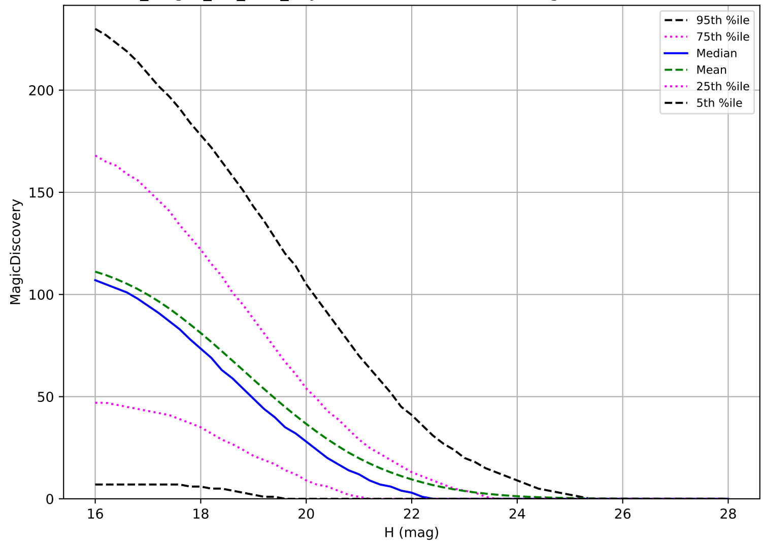
no_magell_roll_v3.4_10yrs: PHA 6 detections in 60 nights detection loss
