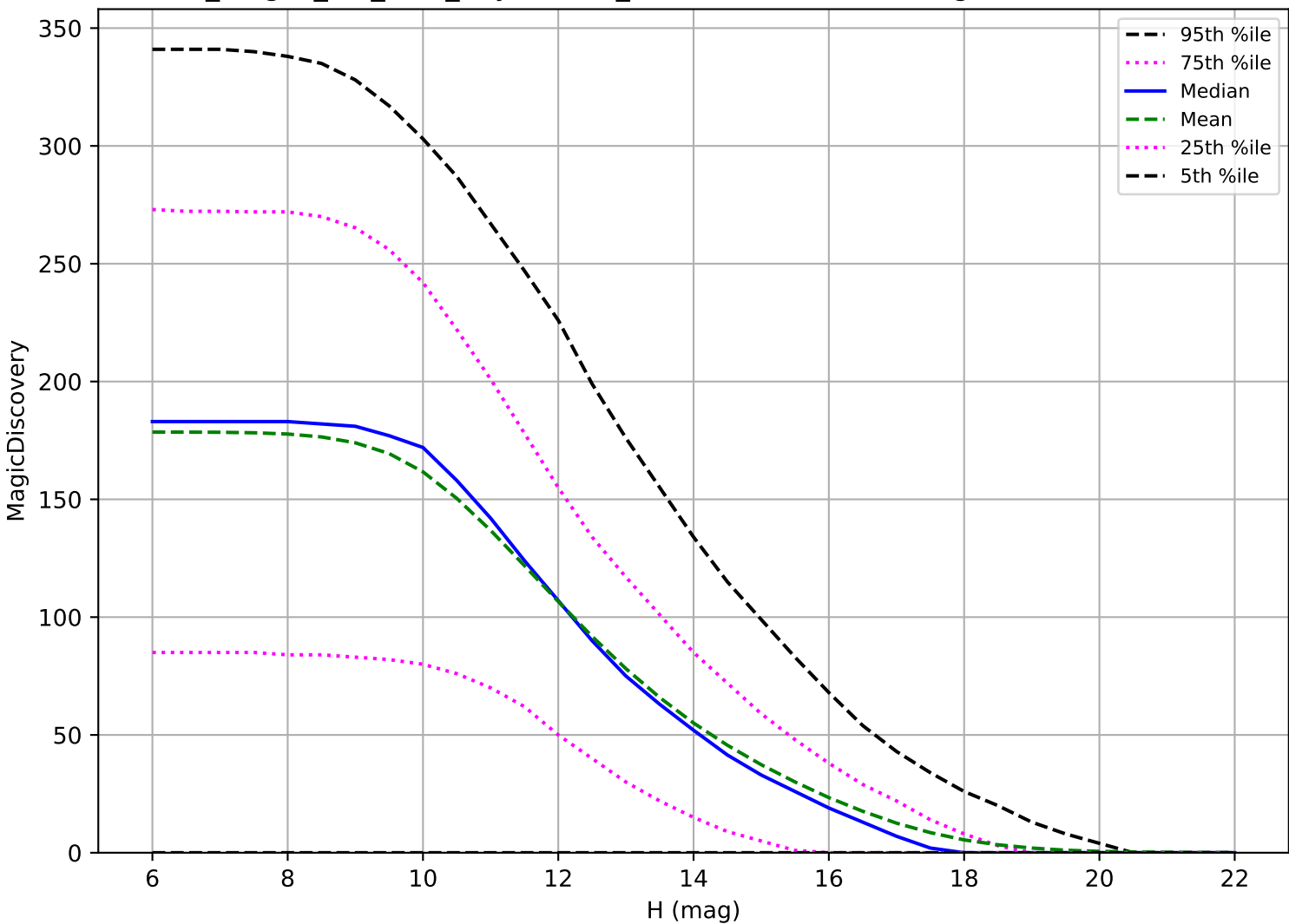
no_magell_roll_v3.4_10yrs: OCC_r5 6 detections in 60 nights detection loss
