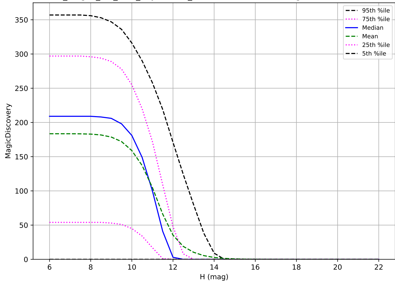
no_magell_roll_v3.4_10yrs: OCC_r20 6 detections in 60 nights detection loss
