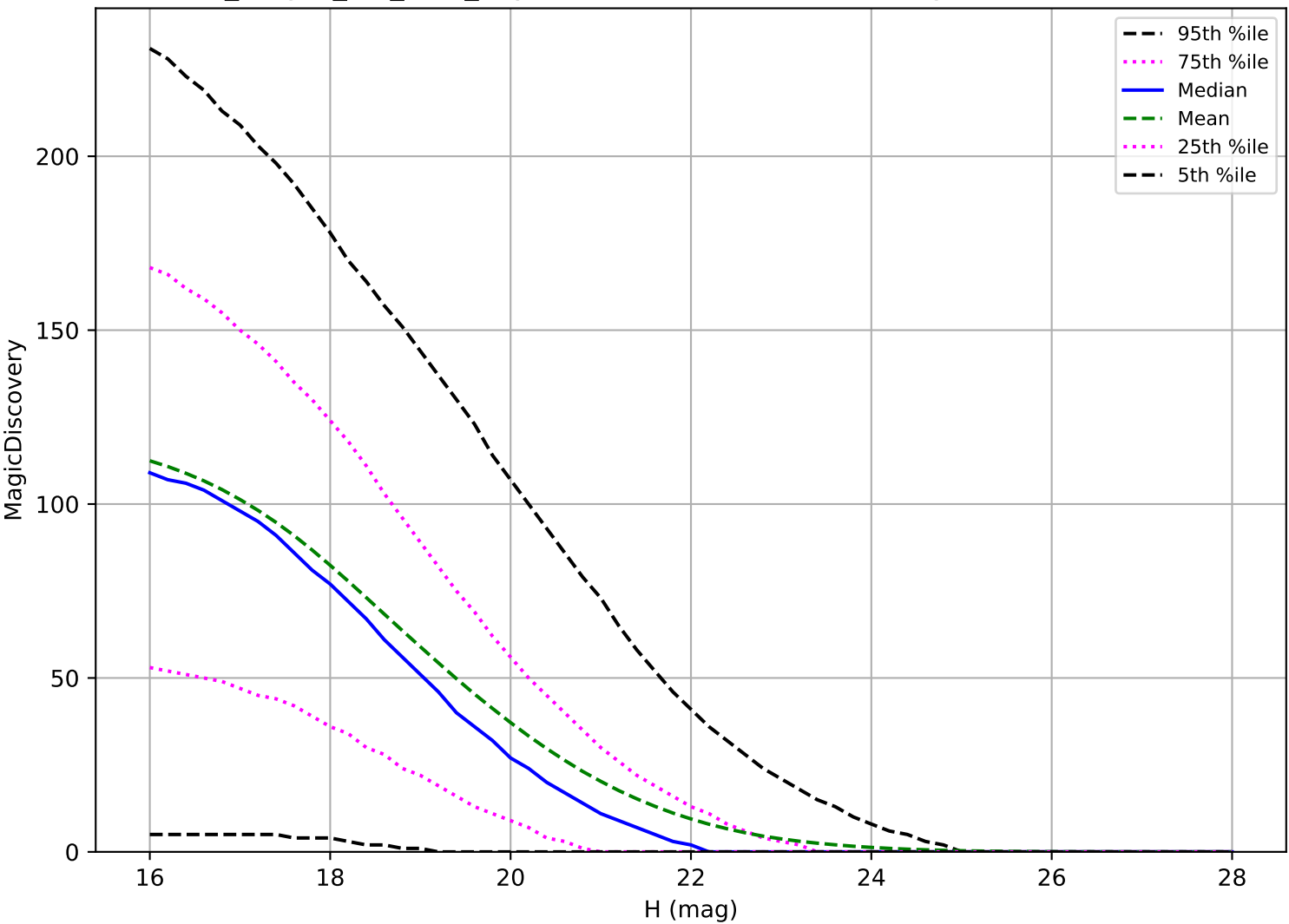
no_magell_roll_v3.4_10yrs: NEO 6 detections in 60 nights detection loss
