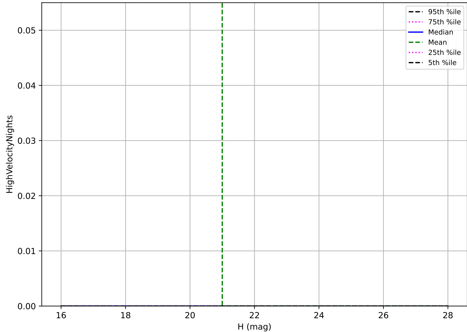
no_magell_roll_v3.4_10yrs: Vatira High velocity pair detection loss
