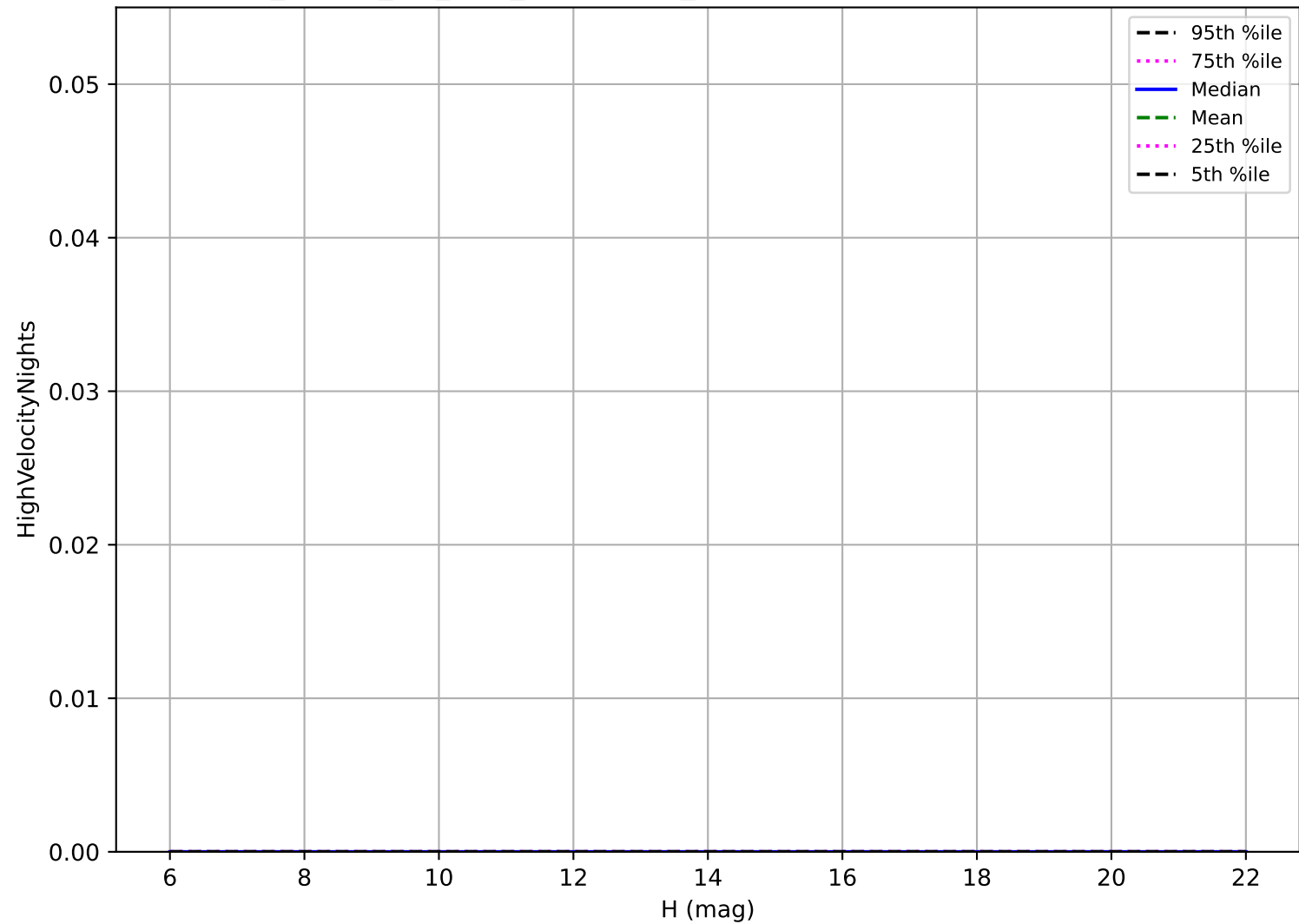
no_magell_roll_v3.4_10yrs: OCC_r5 High velocity pair detection loss
