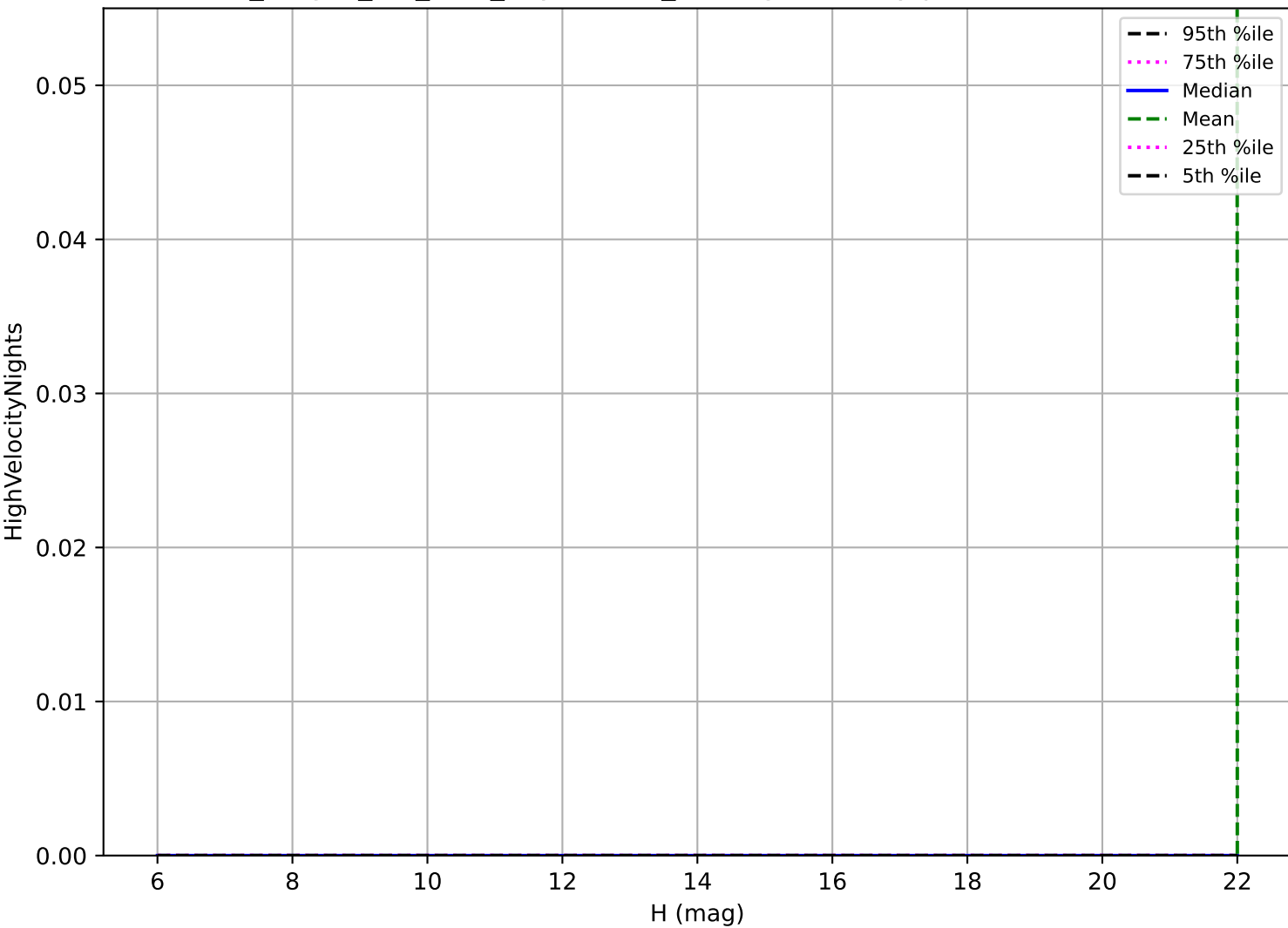
no_magell_roll_v3.4_10yrs: OCC_r20 High velocity pair detection loss
