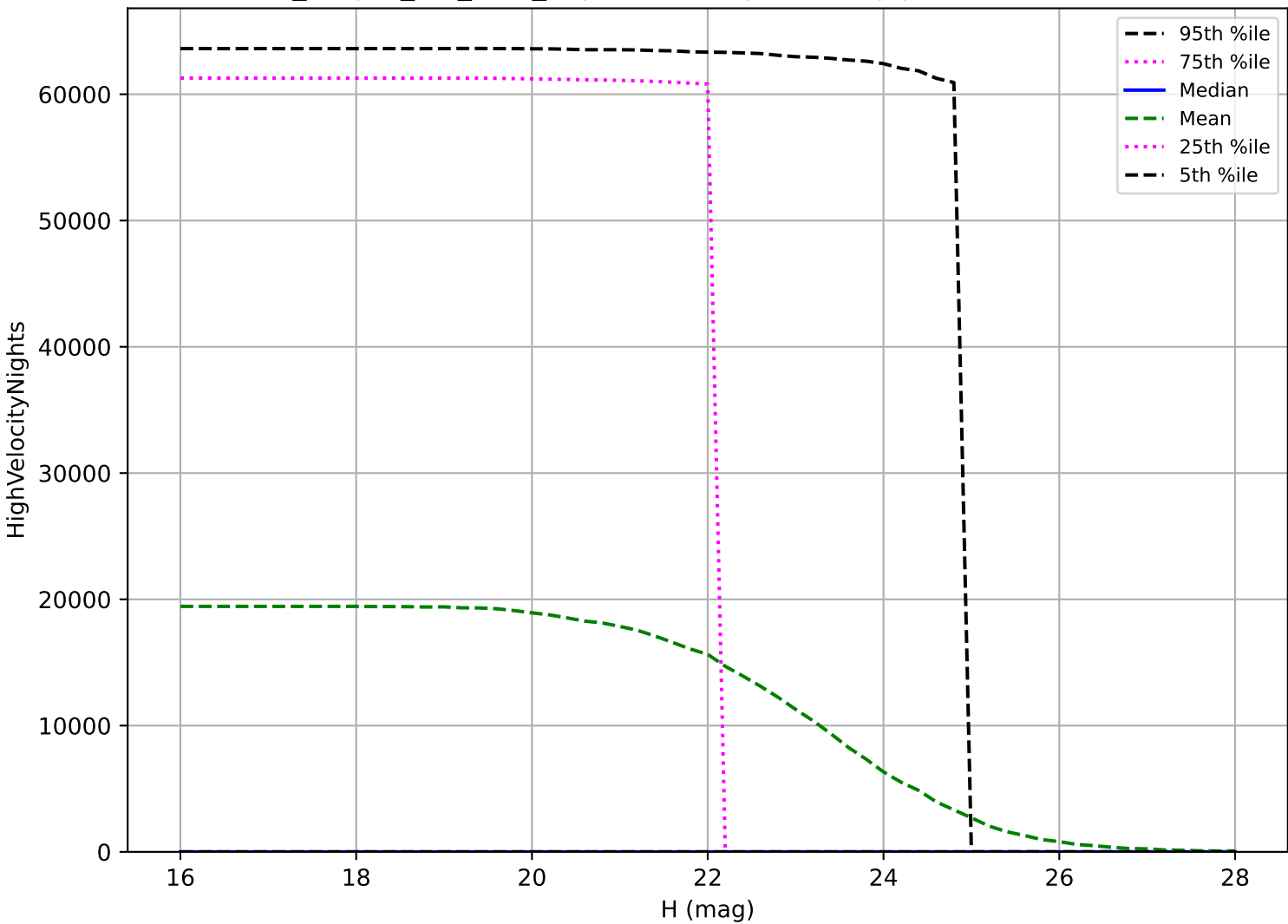
no_magell_roll_v3.4_10yrs: NEO High velocity pair detection loss
