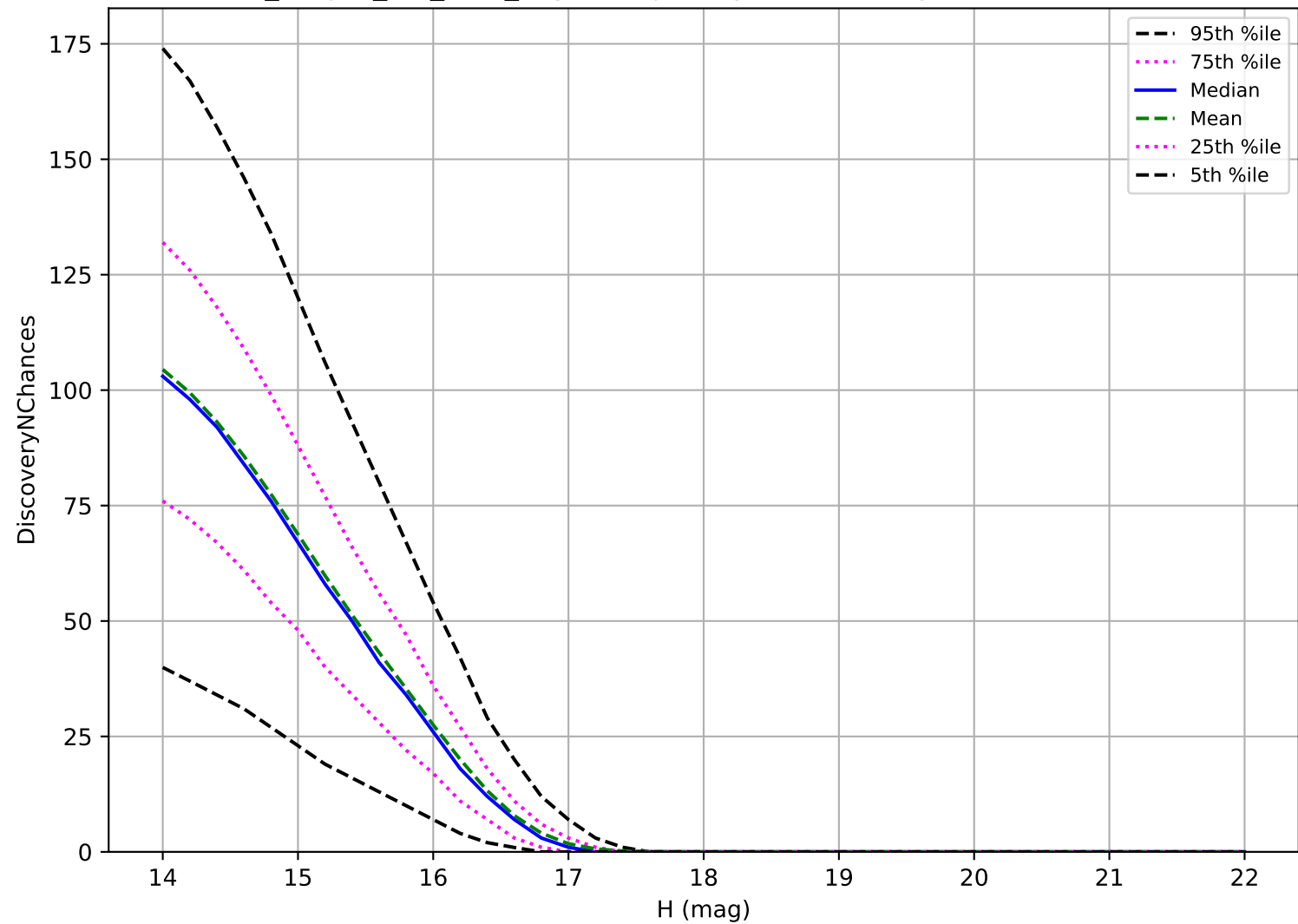
no_magell_roll_v3.4_10yrs: Trojan 3 pairs in 15 nights detection loss
