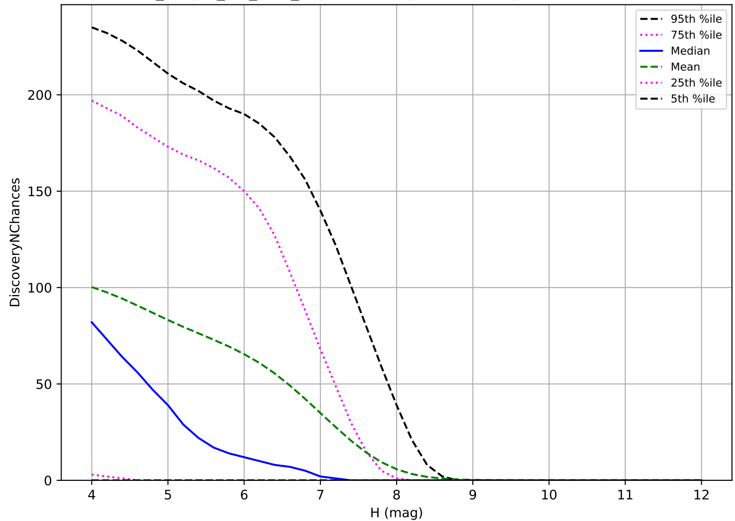
no_magell_roll_v3.4_10yrs: TNO 3 pairs in 15 nights detection loss
