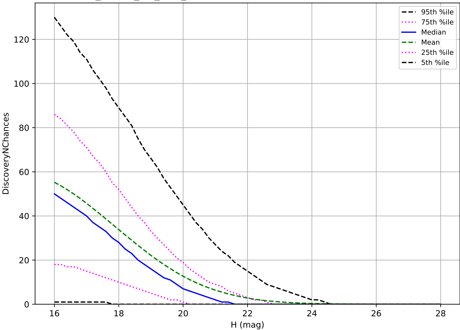
no_magell_roll_v3.4_10yrs: PHA 3 pairs in 15 nights detection loss
