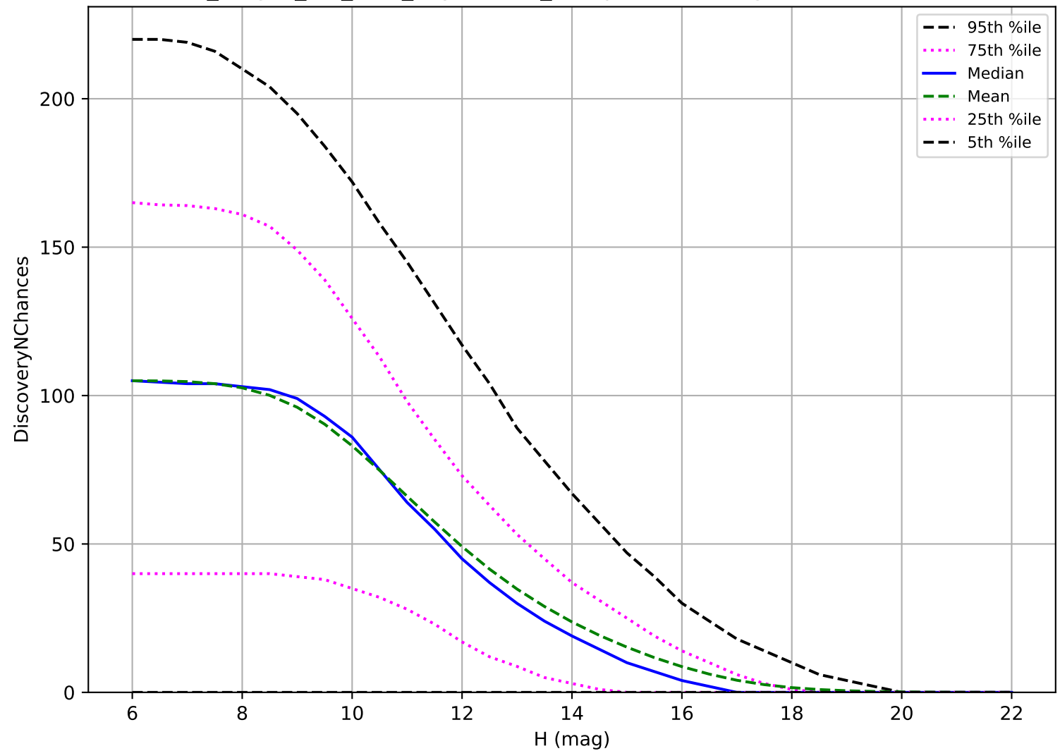
no_magell_roll_v3.4_10yrs: OCC_r5 3 pairs in 15 nights detection loss
