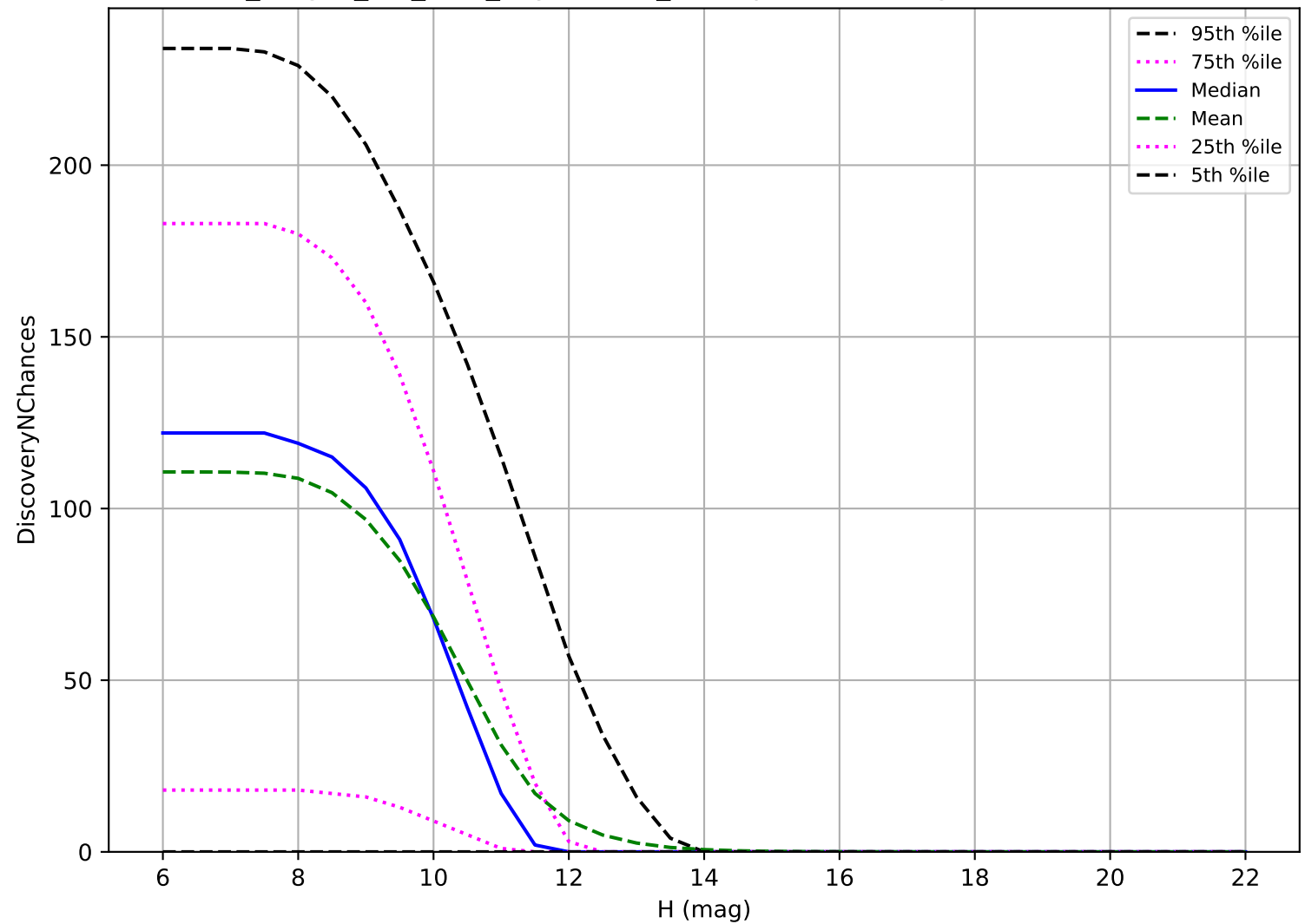
no_magell_roll_v3.4_10yrs: OCC_r20 3 pairs in 15 nights detection loss
