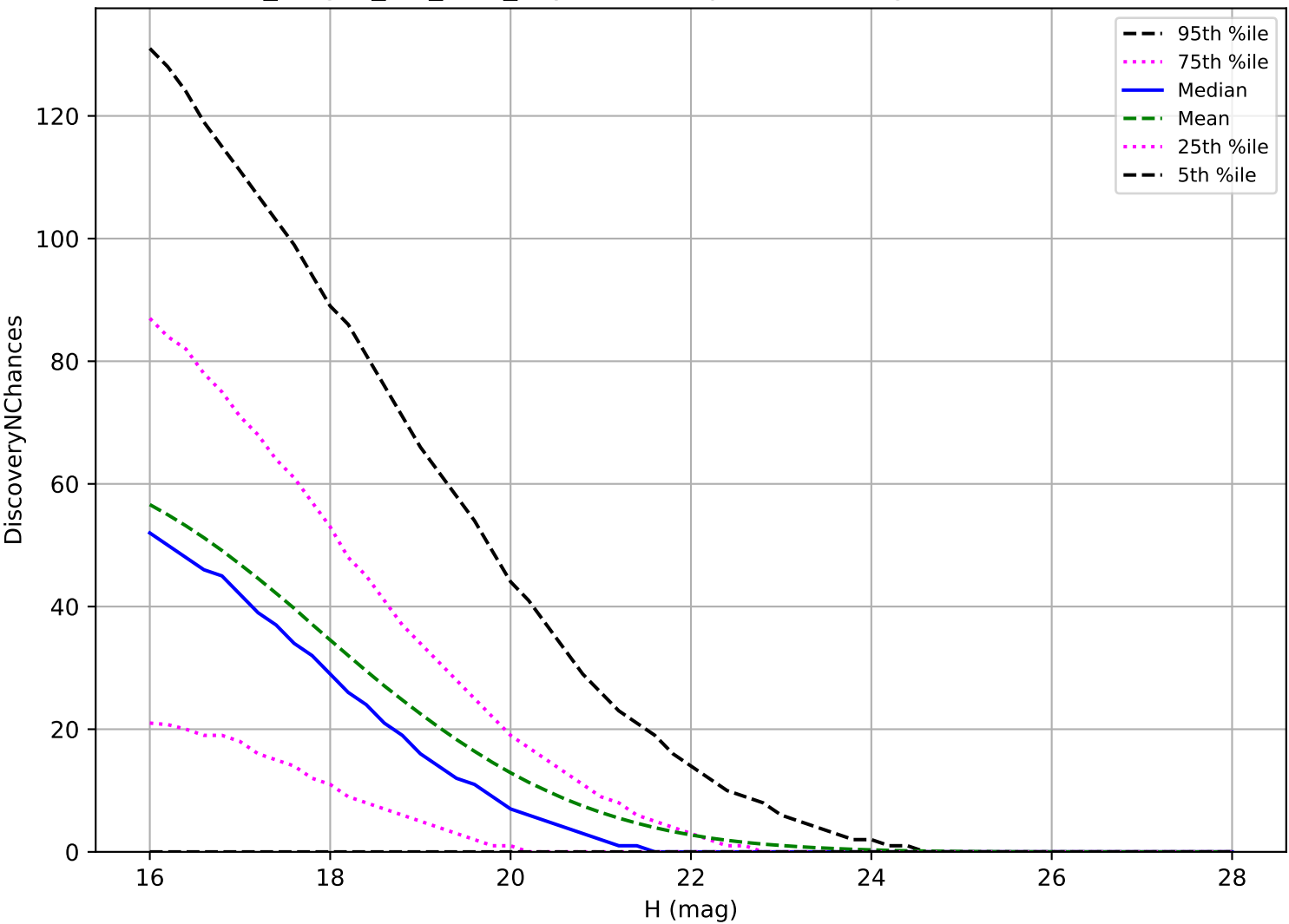
no_magell_roll_v3.4_10yrs: NEO 3 pairs in 15 nights detection loss
