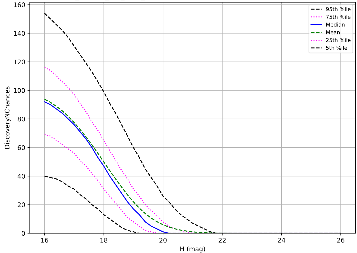
no_magell_roll_v3.4_10yrs: MBA 3 pairs in 15 nights detection loss
