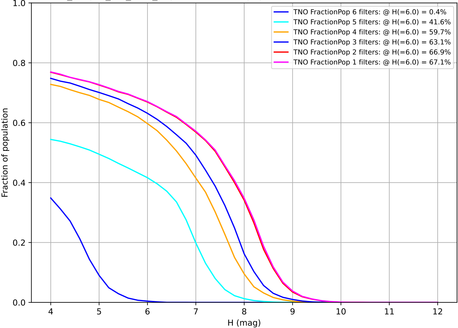
no_magell_roll_v3.4_10yrs: Fraction of population with colors in X filters TNO
