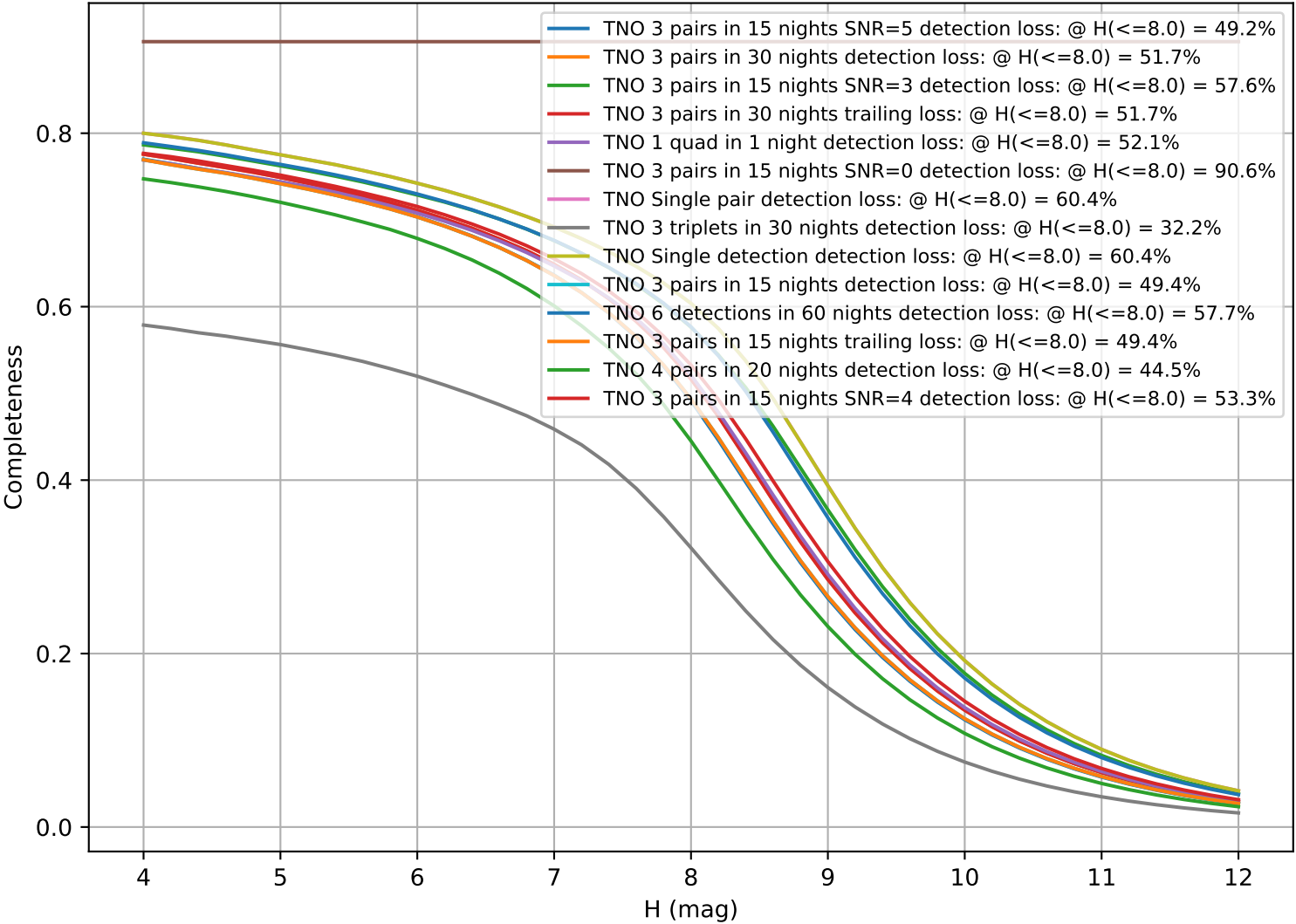
no_magell_roll_v3.4_10yrs: CumulativeCompleteness
