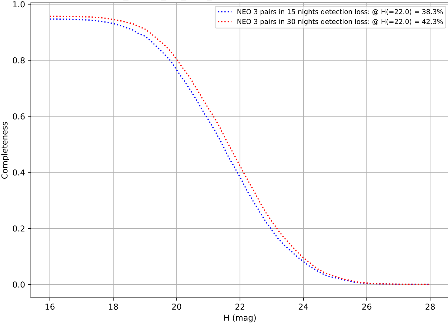
no_magell_roll_v3.4_10yrs: DifferentialCompleteness
