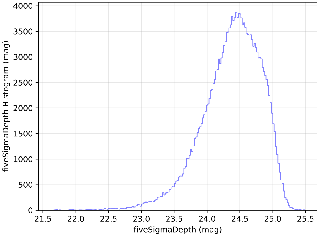
no_magell_roll_v3.4_10yrs g: fiveSigmaDepth Histogram
