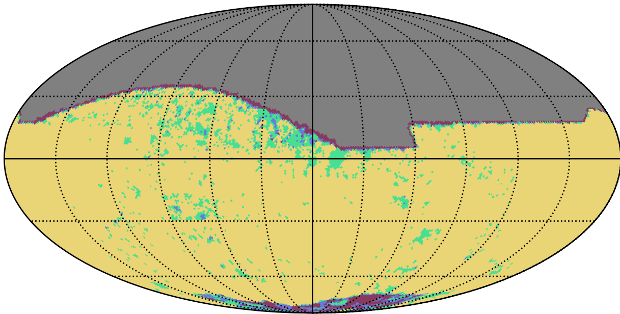
no_magell_roll_v3.4_10yrs z band: YearCoverage night
