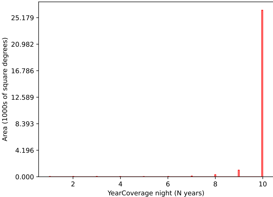
no_magell_roll_v3.4_10yrs i band: YearCoverage night
