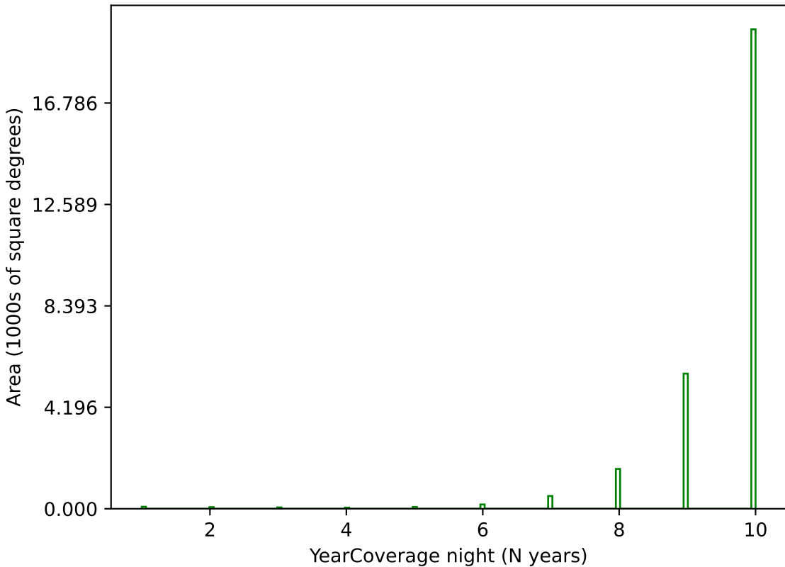
no_magell_roll_v3.4_10yrs g band: YearCoverage night
