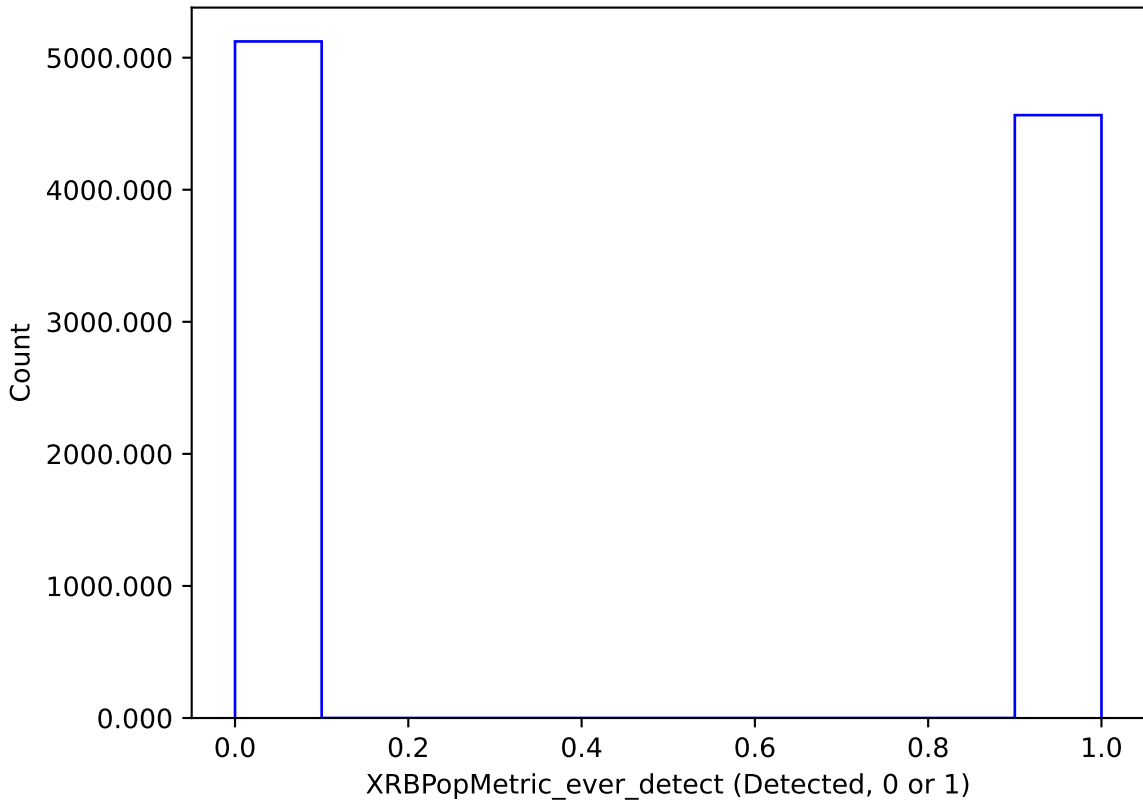
no_magell_roll_v3.4_10yrs : XRBPpopMetric_ever_detect
