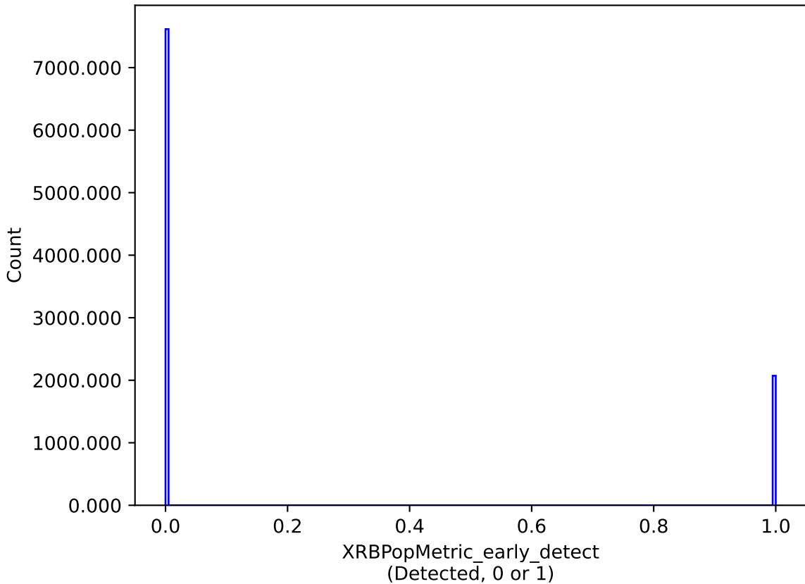
no_magell_roll_v3.4_10yrs : XRBPoMetric_early_detect
