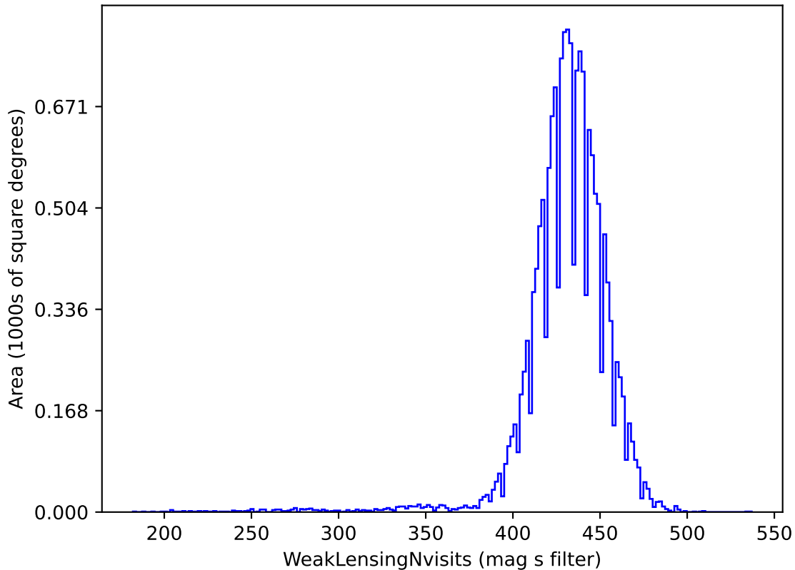
no_magell_roll_v3.4_10yrs gri band non-DD: WeakLensingNvisits
