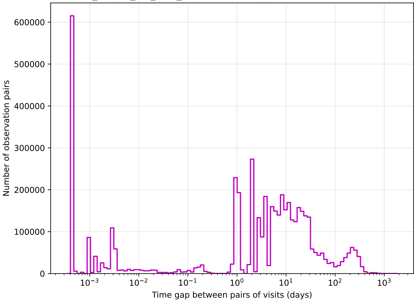
no_magell_roll_v3.4_10yrs z band: Tgaps observationStartMJD
