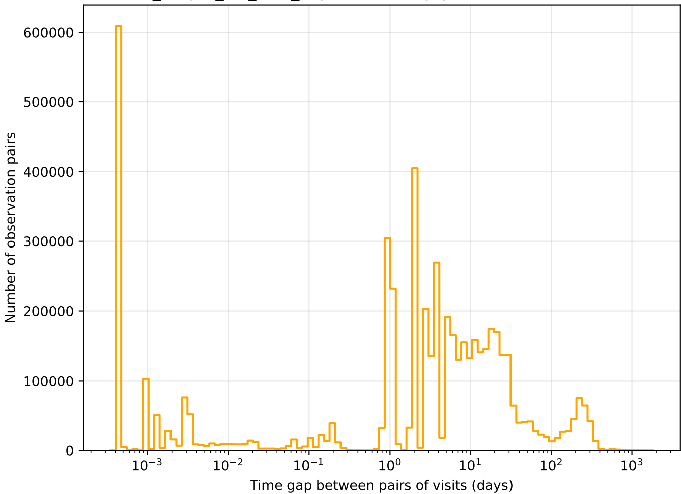
no_magell_roll_v3.4_10yrs r band: Tgaps observationStartMJD
