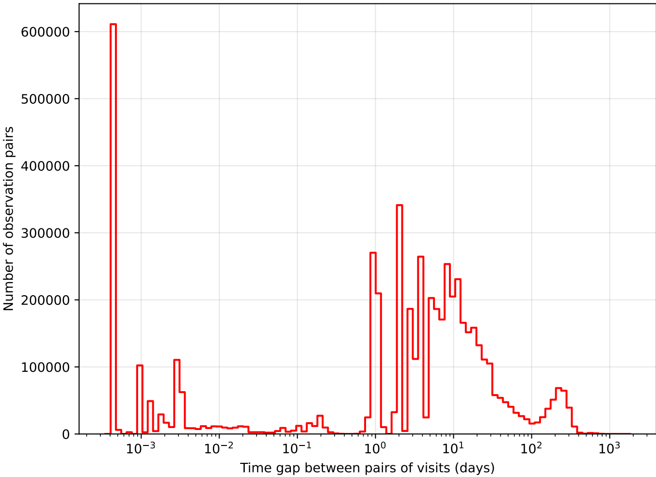
no_magell_roll_v3.4_10yrs i band: Tgaps observationStartMJD
