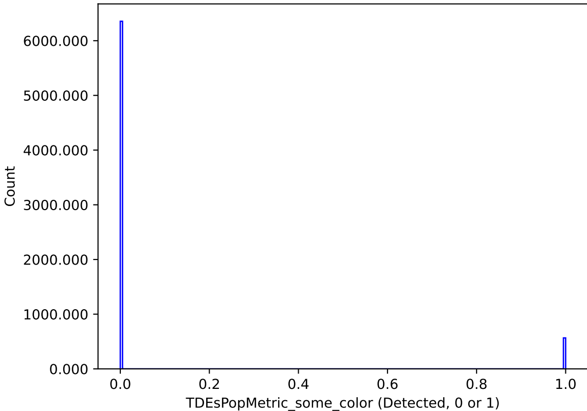
no_magell_roll_v3.4_10yrs : TDEsPopMetric_some_color
