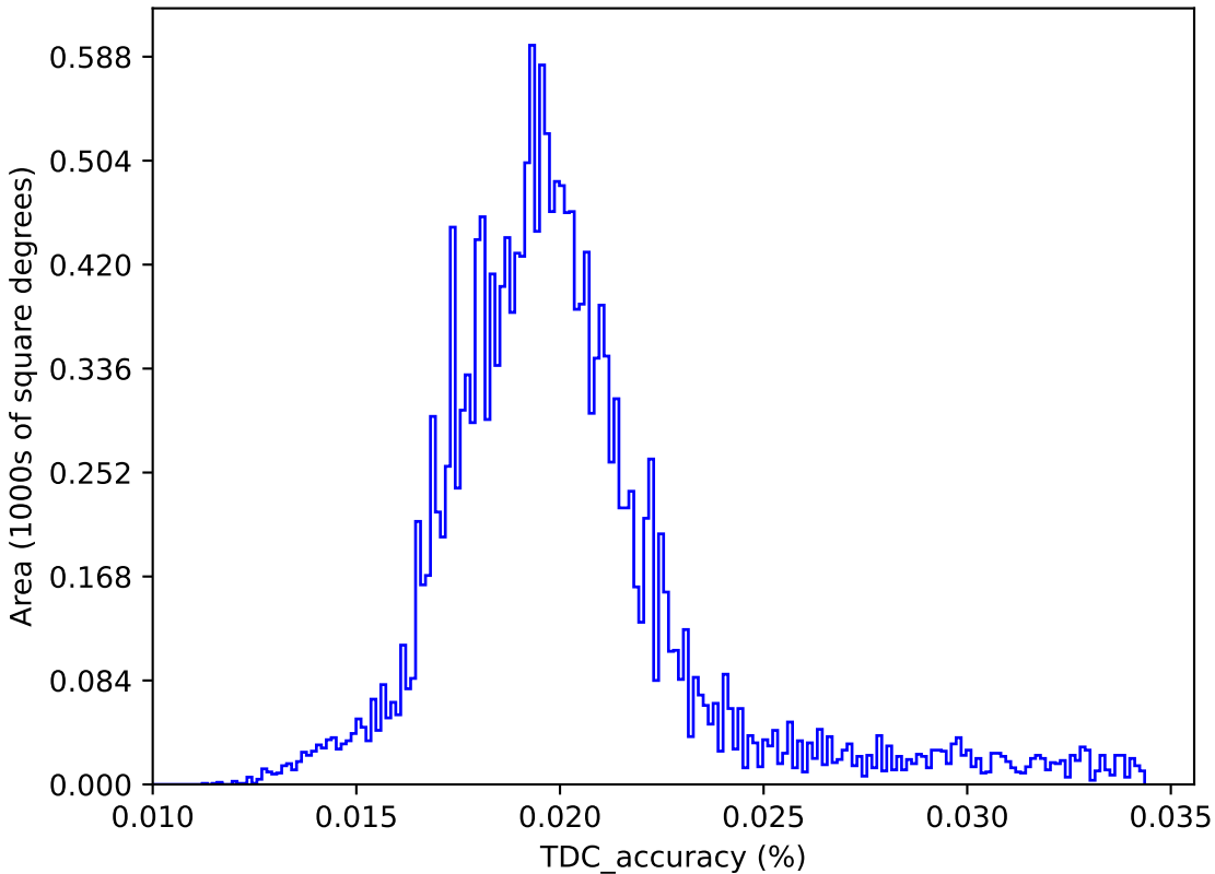
no_magell_roll_v3.4_10yrs : TDC_accuracy
