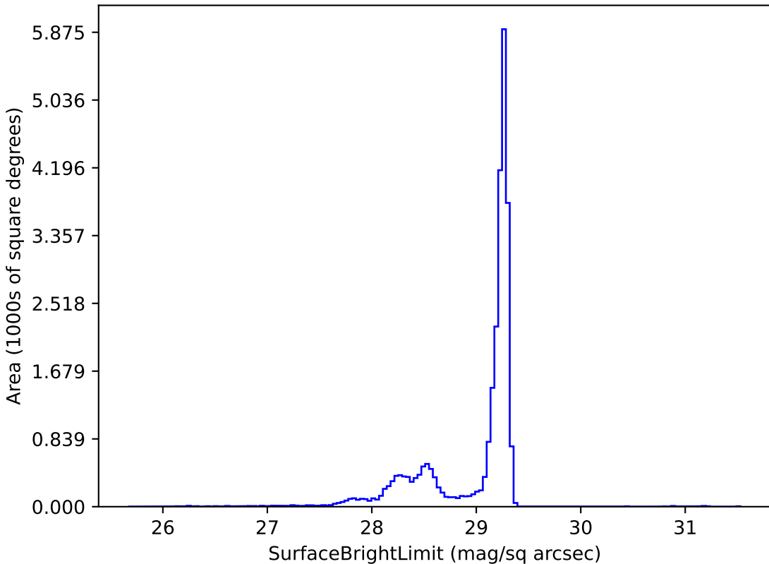
no_magell_roll_v3.4_10yrs z: SurfaceBrightLimit
