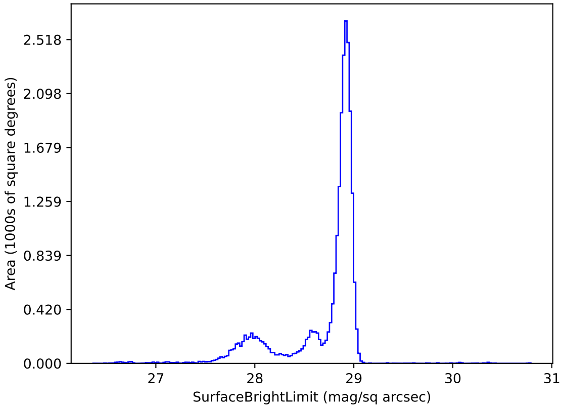
no_magell_roll_v3.4_10yrs u: SurfaceBrightLimit
