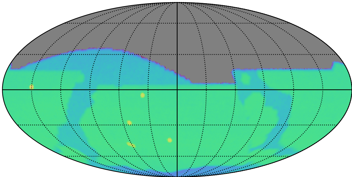
no_magell_roll_v3.4_10yrs r: SurfaceBrightLimit
