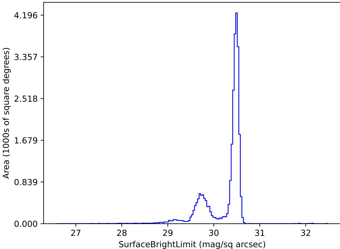
no_magell_roll_v3.4_10yrs r: SurfaceBrightLimit
