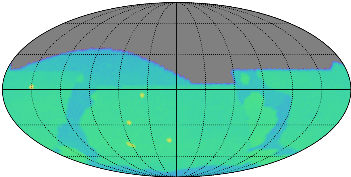
no_magell_roll_v3.4_10yrs g: SurfaceBrightLimit
