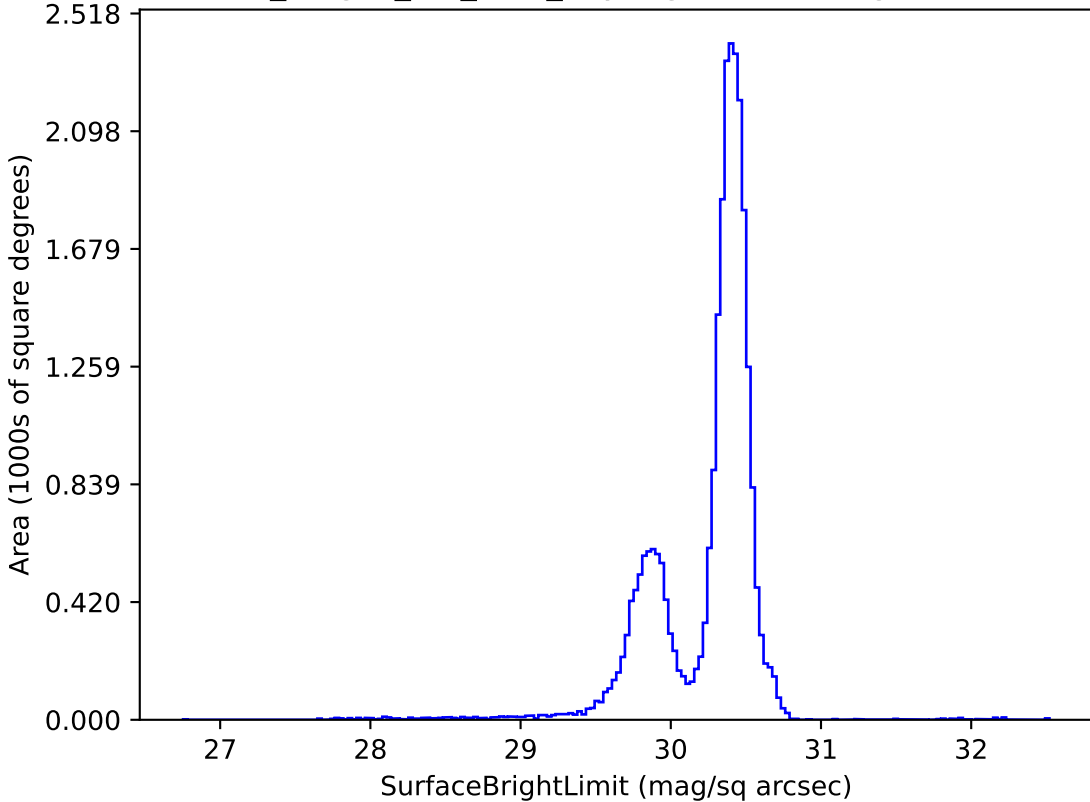
no_magell_roll_v3.4_10yrs g: SurfaceBrightLimit
